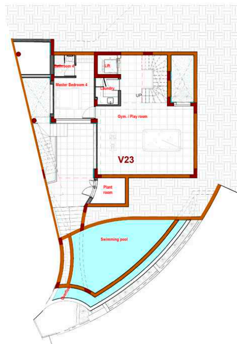
LOWER GROUND FLOOR PLAN LEVEL 2
